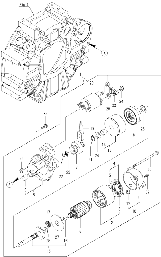
OCD50-M00220 3TNM72-HHFCG Fig.15. STARTING MOTOR
