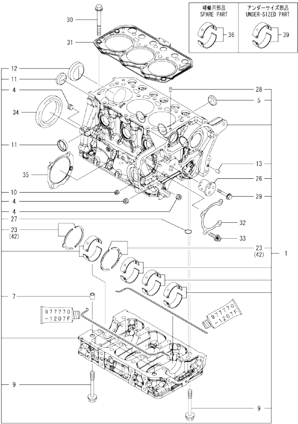
OCD50-M00220 3TNM72-HHFCG Fig.1. CYLINDER BLOCK
