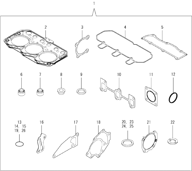
Fig.17. GASKET SET
