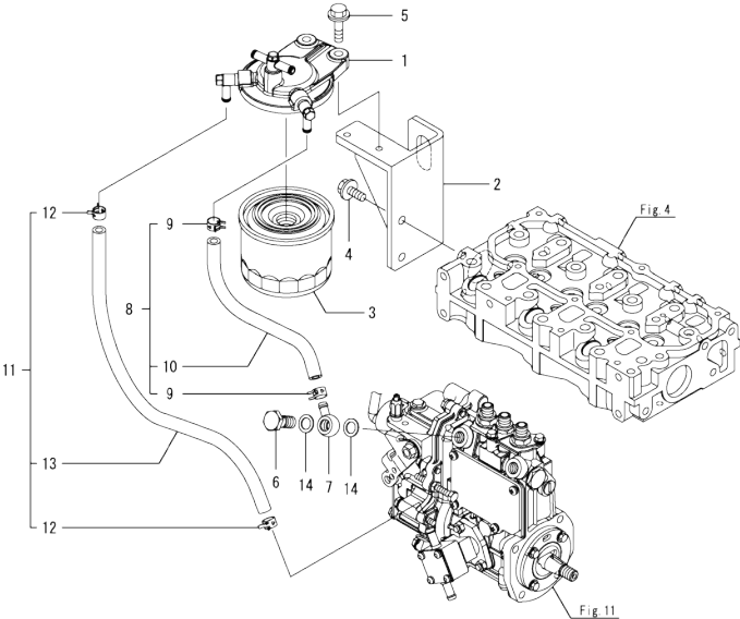
Fig.14. FUEL PIPE
