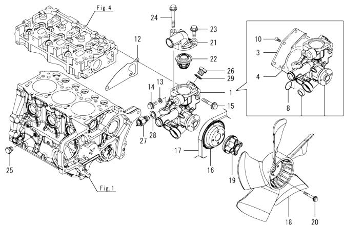
Fig.10. COOLING WATER SYSTEM
